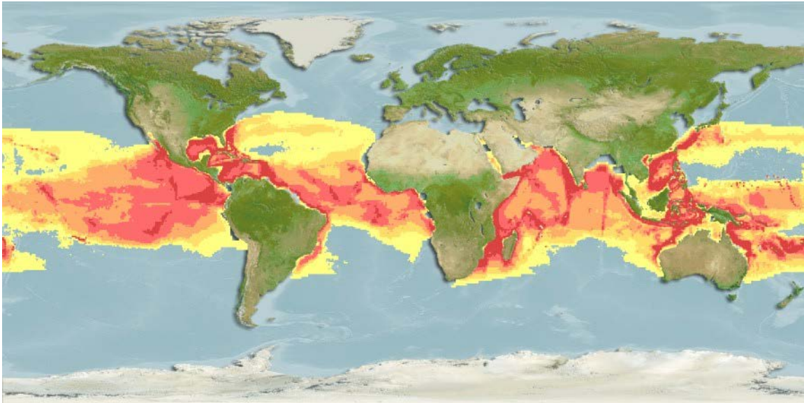
Figure 1: Expert reviewed AquaMaps predictions: Melon-headed whale ( Peponocephala electra )
